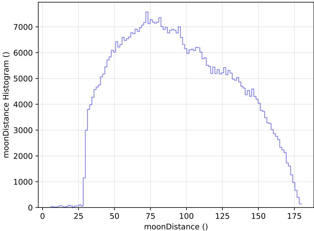
extra_ss_neo2_v3.4_10yrs All sky i band: moonDistance Histogram
