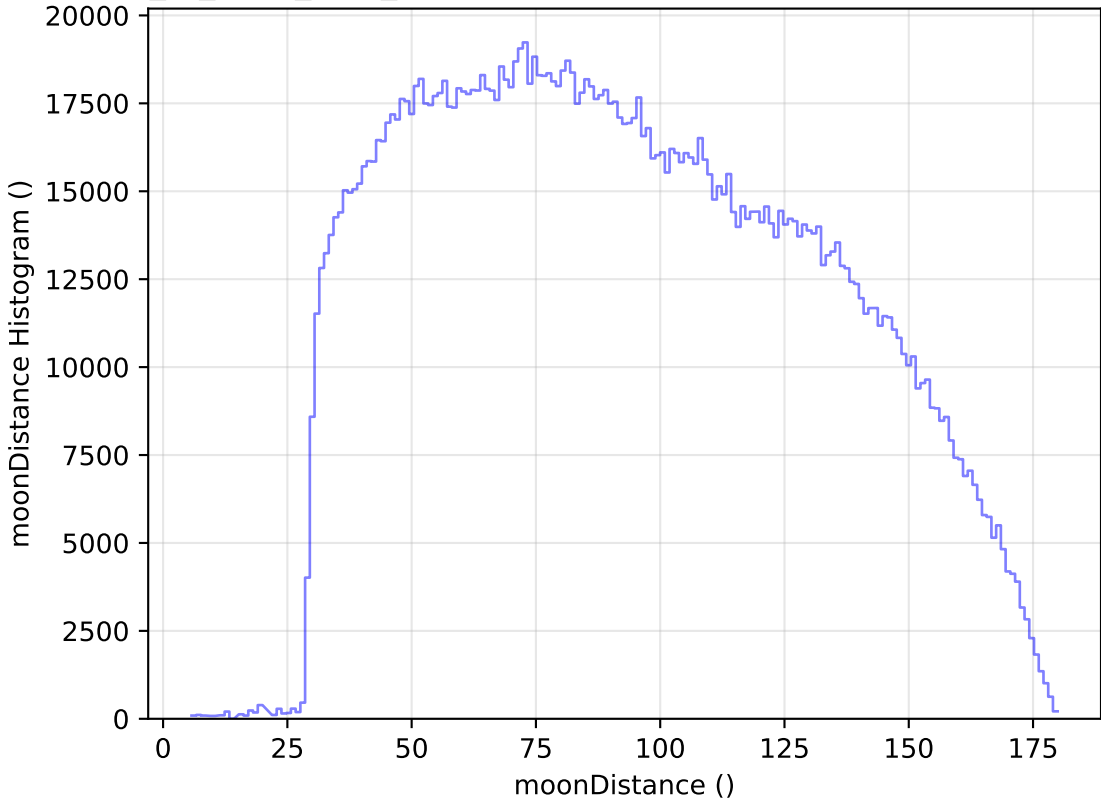
extra_ss_neo2_v3.4_10yrs All sky all bands: moonDistance Histogram
