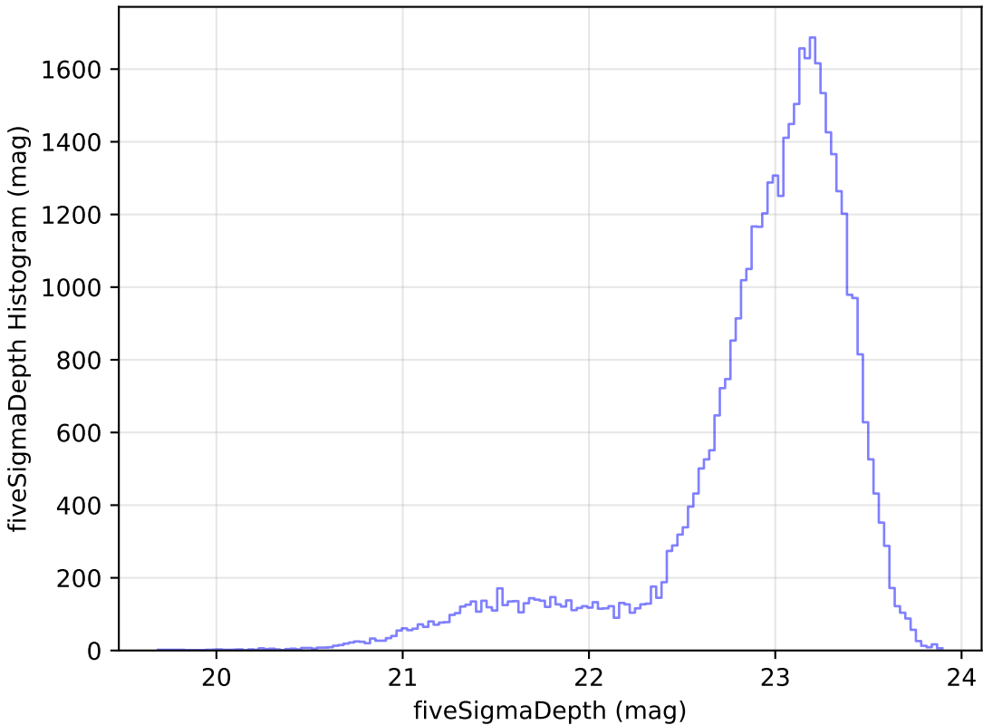
extra_ss_neo2_v3.4_10yrs Yr 1 z band: fiveSigmaDepth Histogram
