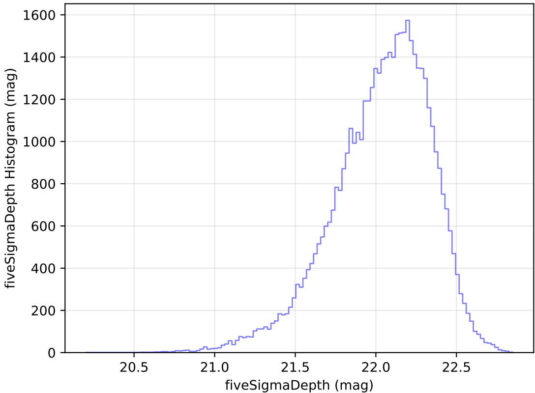
extra_ss_neo2_v3.4_10yrs Yr 1 y band: fiveSigmaDepth Histogram
