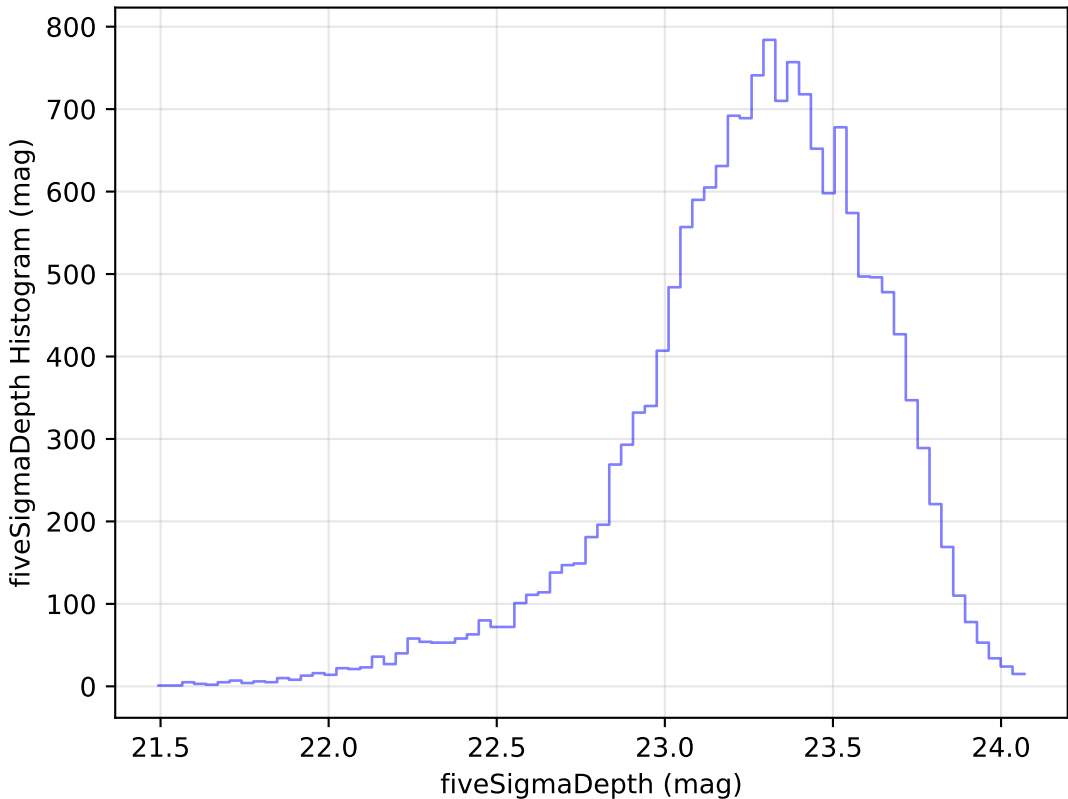
extra_ss_neo2_v3.4_10yrs Yr 1 u band: fiveSigmaDepth Histogram
