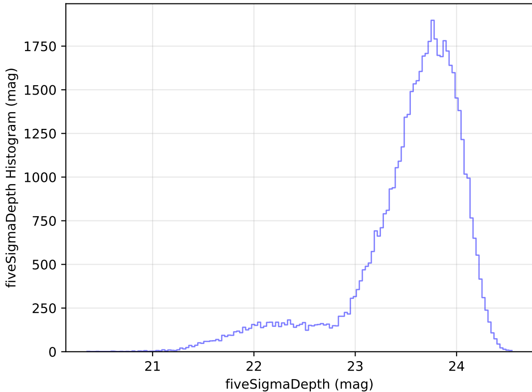
extra_ss_neo2_v3.4_10yrs Yr 1 i band: fiveSigmaDepth Histogram
