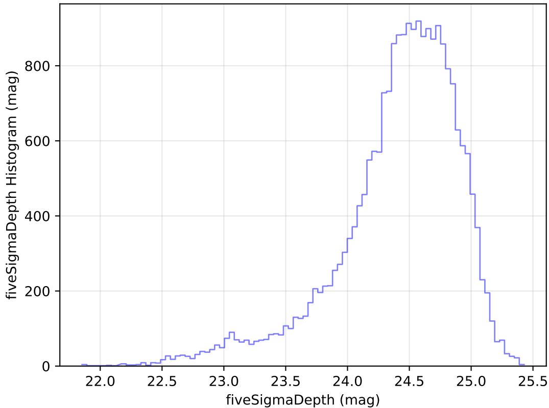
extra_ss_neo2_v3.4_10yrs Yr 1 g band: fiveSigmaDepth Histogram
