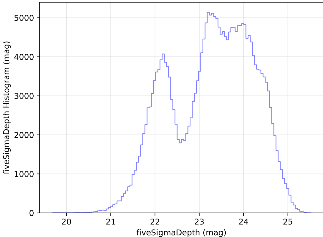
extra_ss_neo2_v3.4_10yrs Yr 1 all bands: fiveSigmaDepth Histogram
