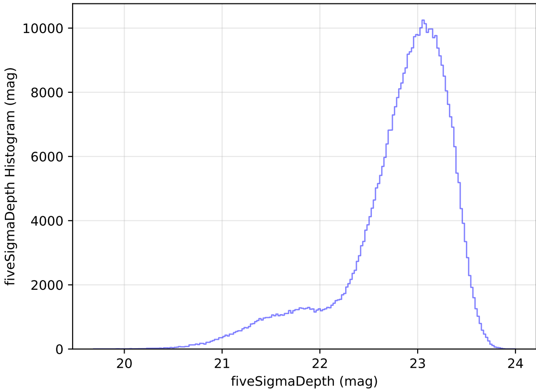
extra_ss_neo2_v3.4_10yrs WFD z band: fiveSigmaDepth Histogram
