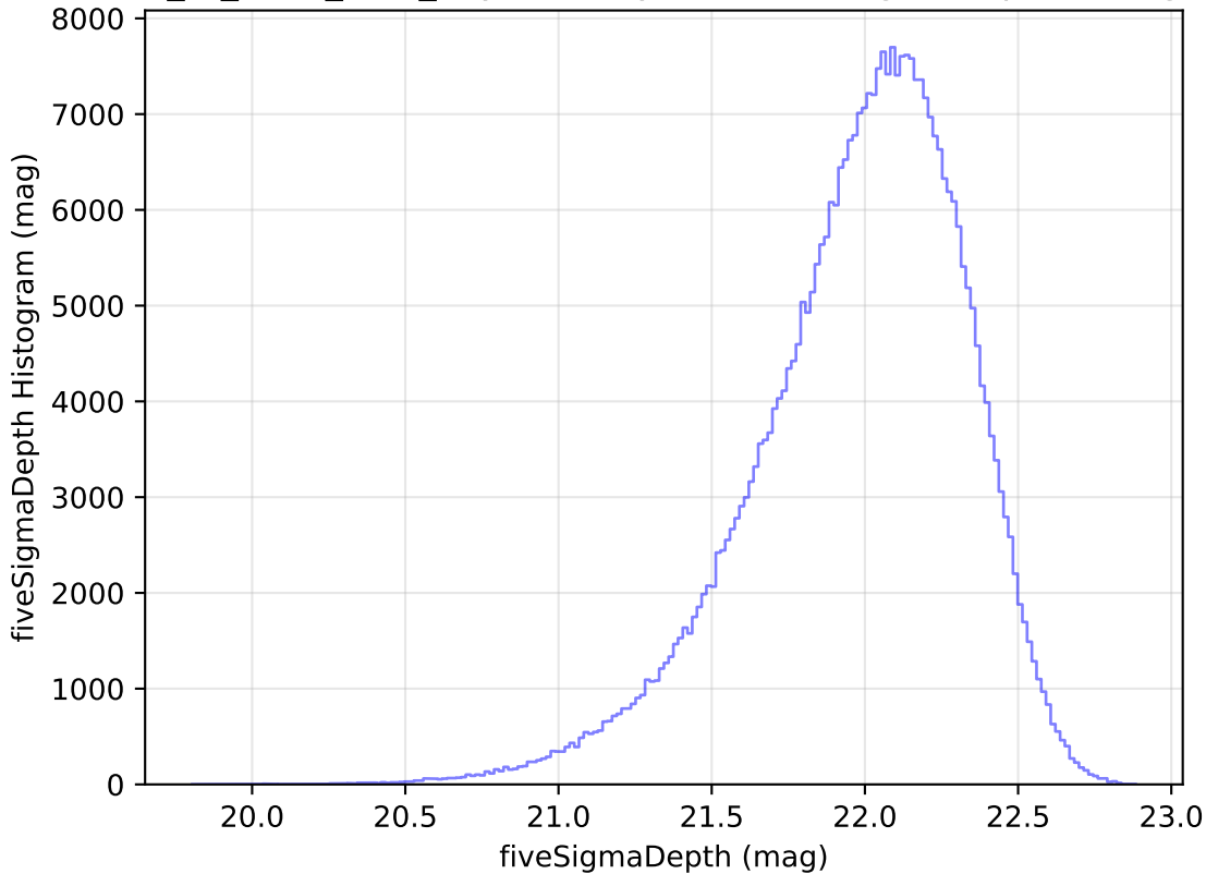
extra_ss_neo2_v3.4_10yrs WFD y band: fiveSigmaDepth Histogram
