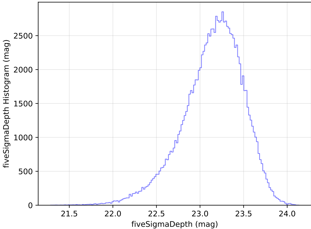
extra_ss_neo2_v3.4_10yrs WFD u band: fiveSigmaDepth Histogram
