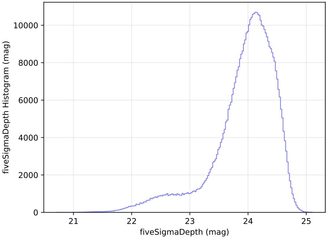
extra_ss_neo2_v3.4_10yrs WFD r band: fiveSigmaDepth Histogram
