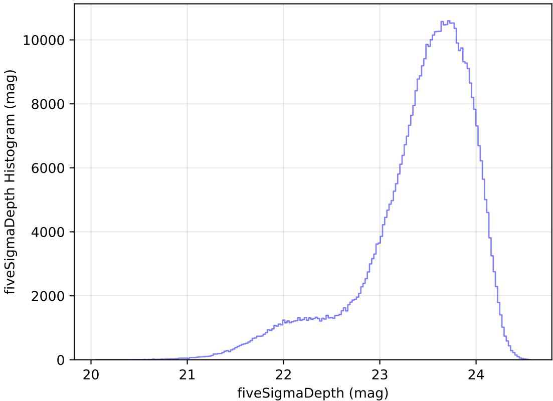
extra_ss_neo2_v3.4_10yrs WFD i band: fiveSigmaDepth Histogram
