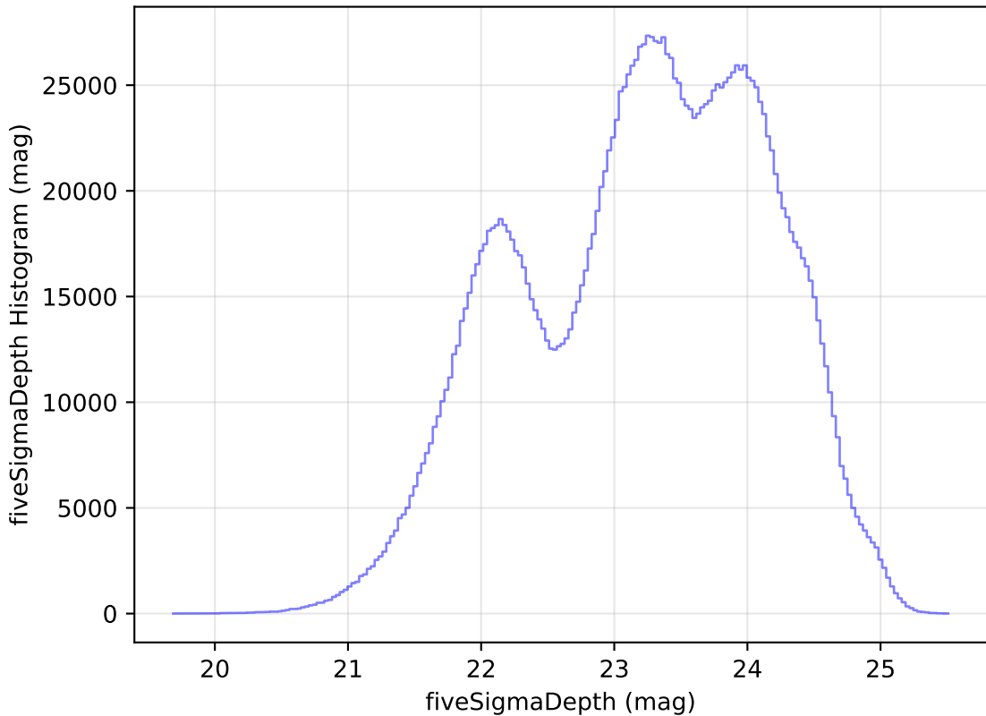
extra_ss_neo2_v3.4_10yrs WFD all bands: fiveSigmaDepth Histogram
