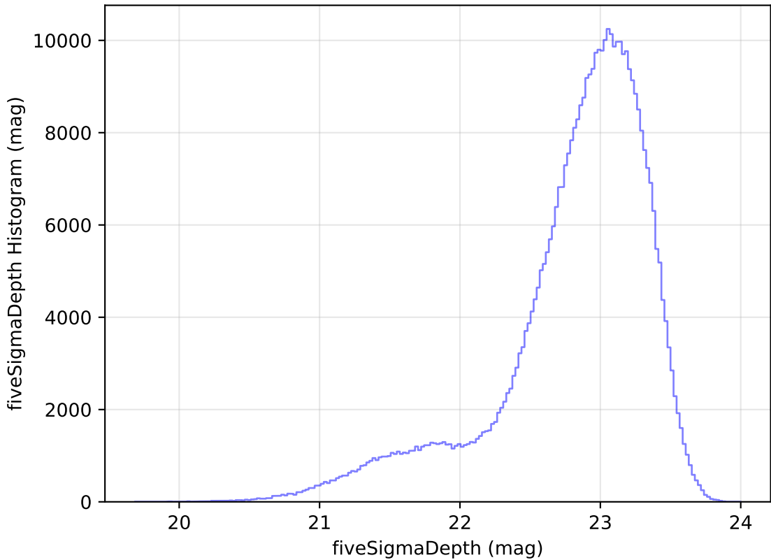
extra_ss_neo2_v3.4_10yrs All sky z band: fiveSigmaDepth Histogram
