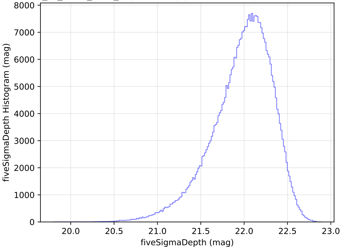
extra_ss_neo2_v3.4_10yrs All sky y band: fiveSigmaDepth Histogram
