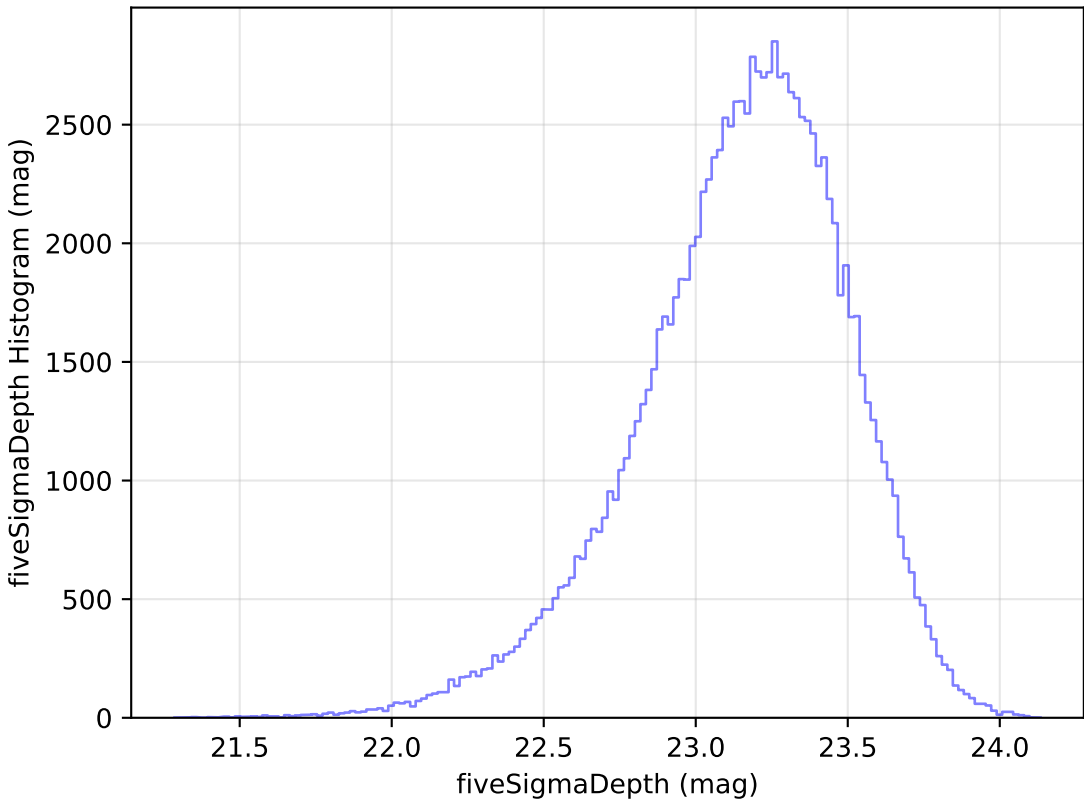
extra_ss_neo2_v3.4_10yrs All sky u band: fiveSigmaDepth Histogram
