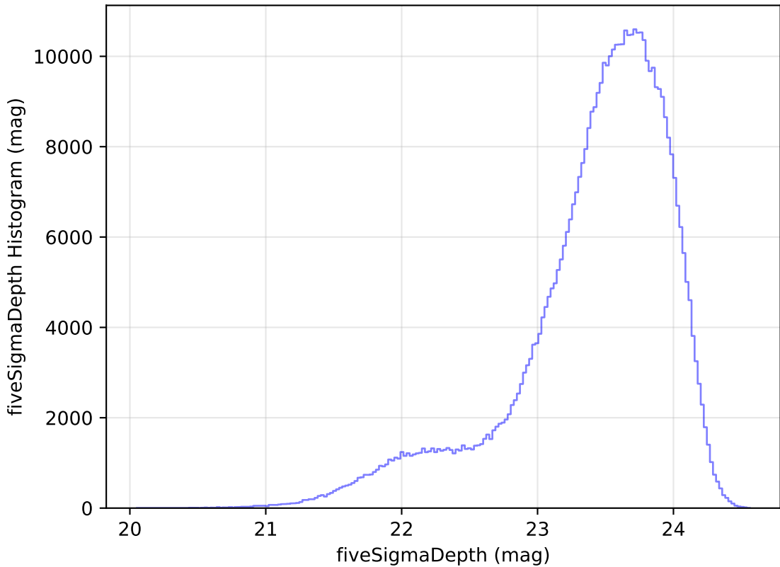
extra_ss_neo2_v3.4_10yrs All sky i band: fiveSigmaDepth Histogram
