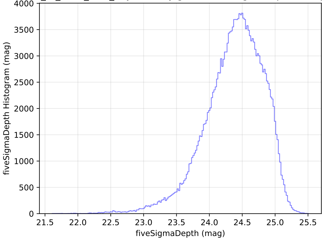
extra_ss_neo2_v3.4_10yrs All sky g band: fiveSigmaDepth Histogram
