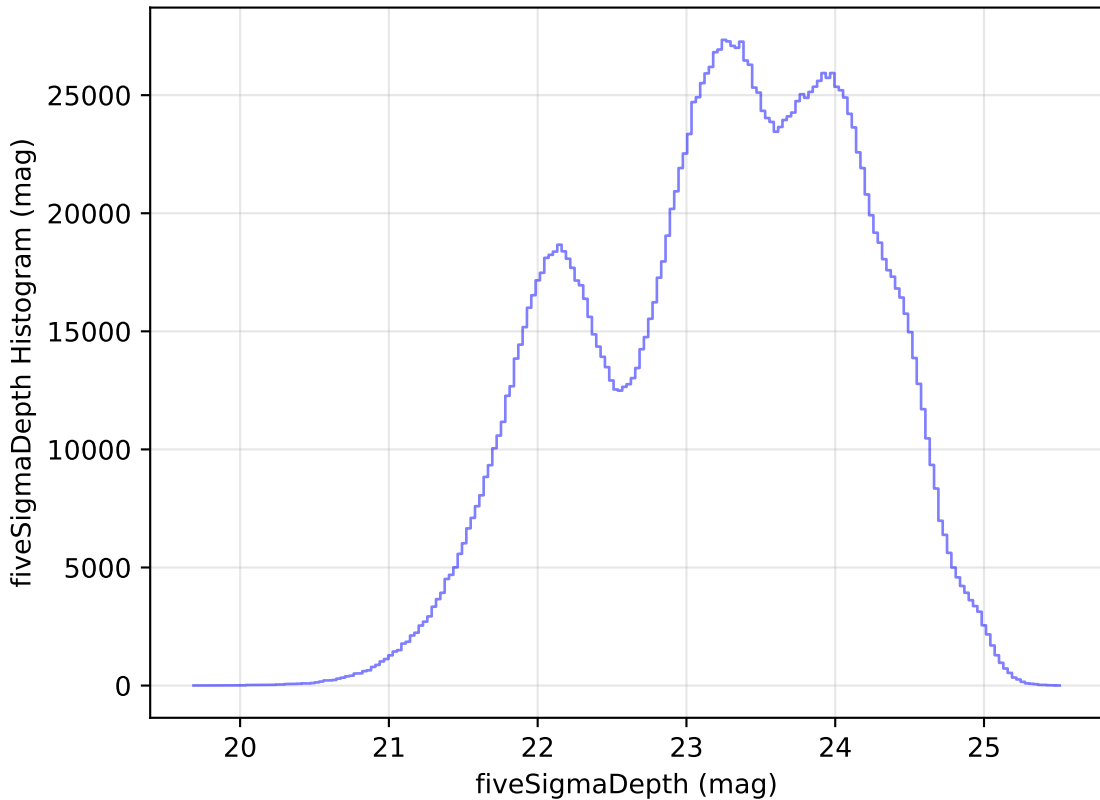
extra_ss_neo2_v3.4_10yrs All sky all bands: fiveSigmaDepth Histogram
