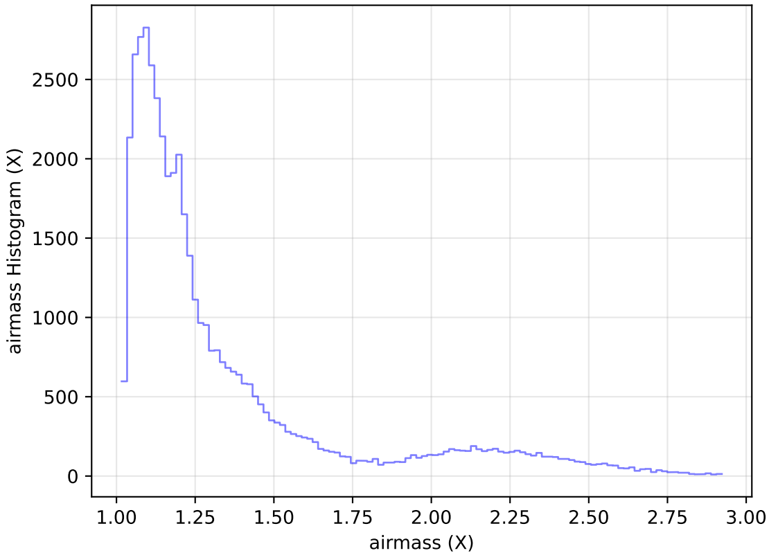
extra_ss_neo2_v3.4_10yrs Yr 1 z band: airmass Histogram
