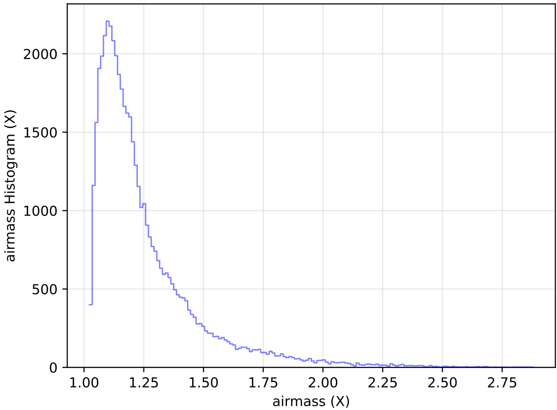
extra_ss_neo2_v3.4_10yrs Yr 1 y band: airmass Histogram
