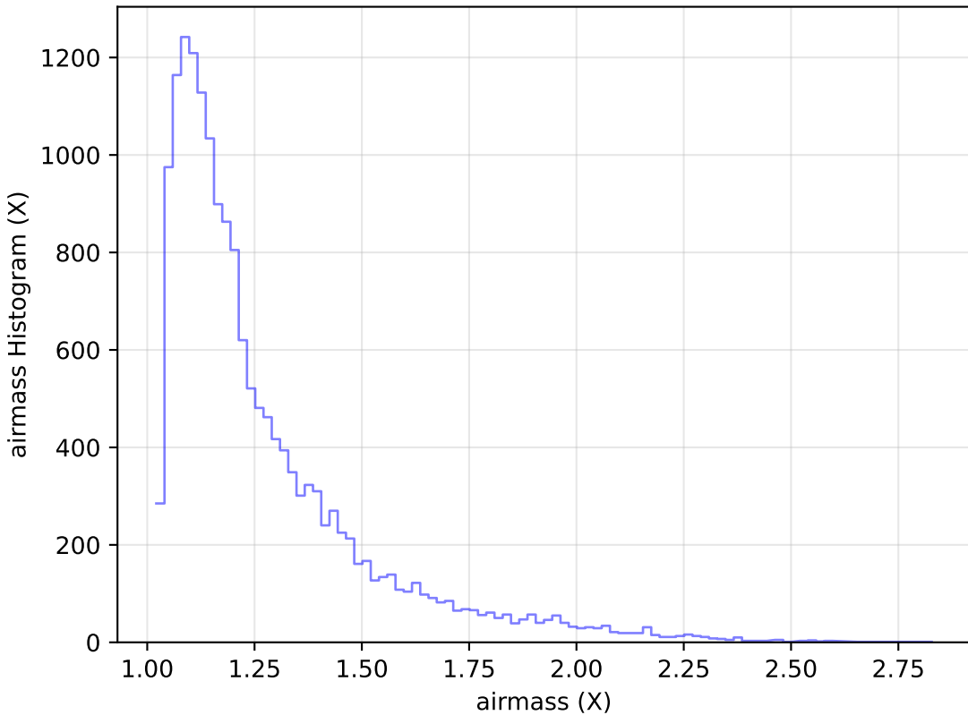
extra_ss_neo2_v3.4_10yrs Yr 1 u band: airmass Histogram
