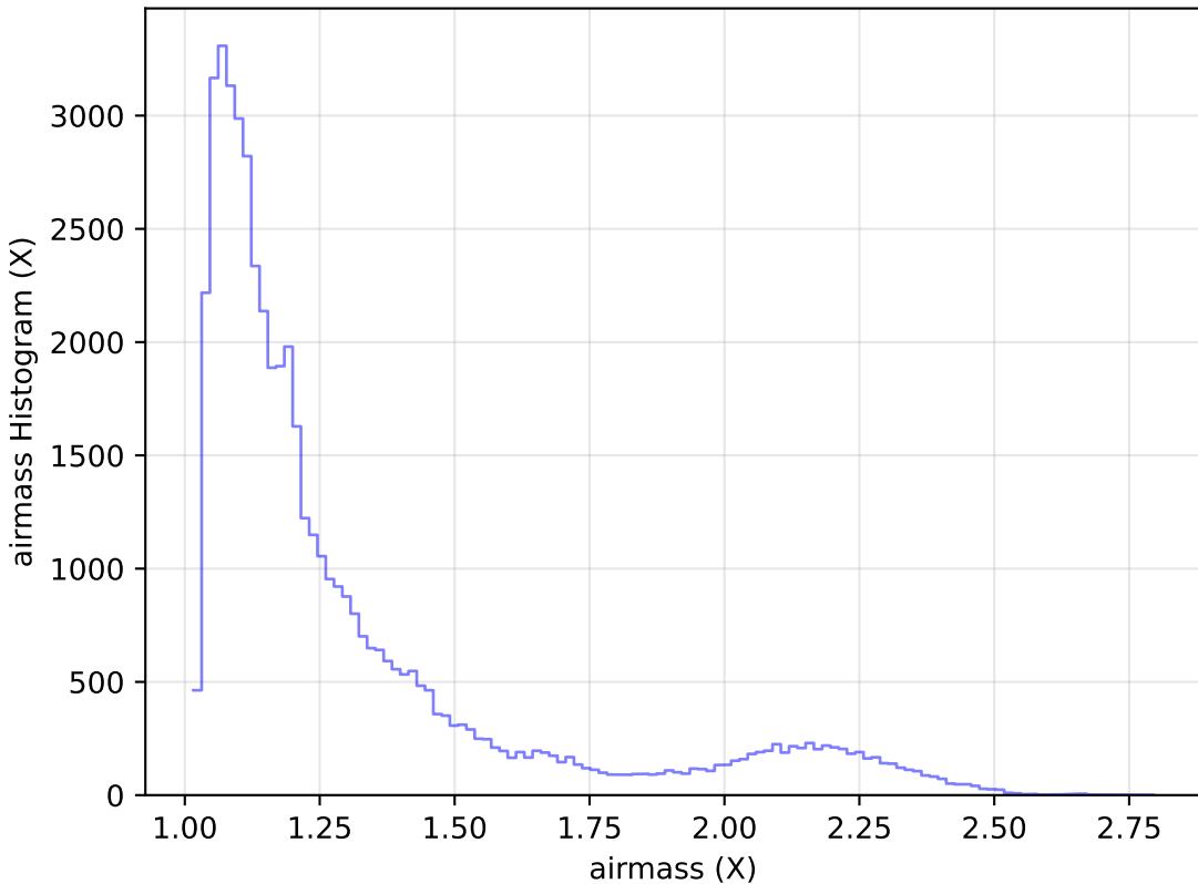
extra_ss_neo2_v3.4_10yrs Yr 1 r band: airmass Histogram
