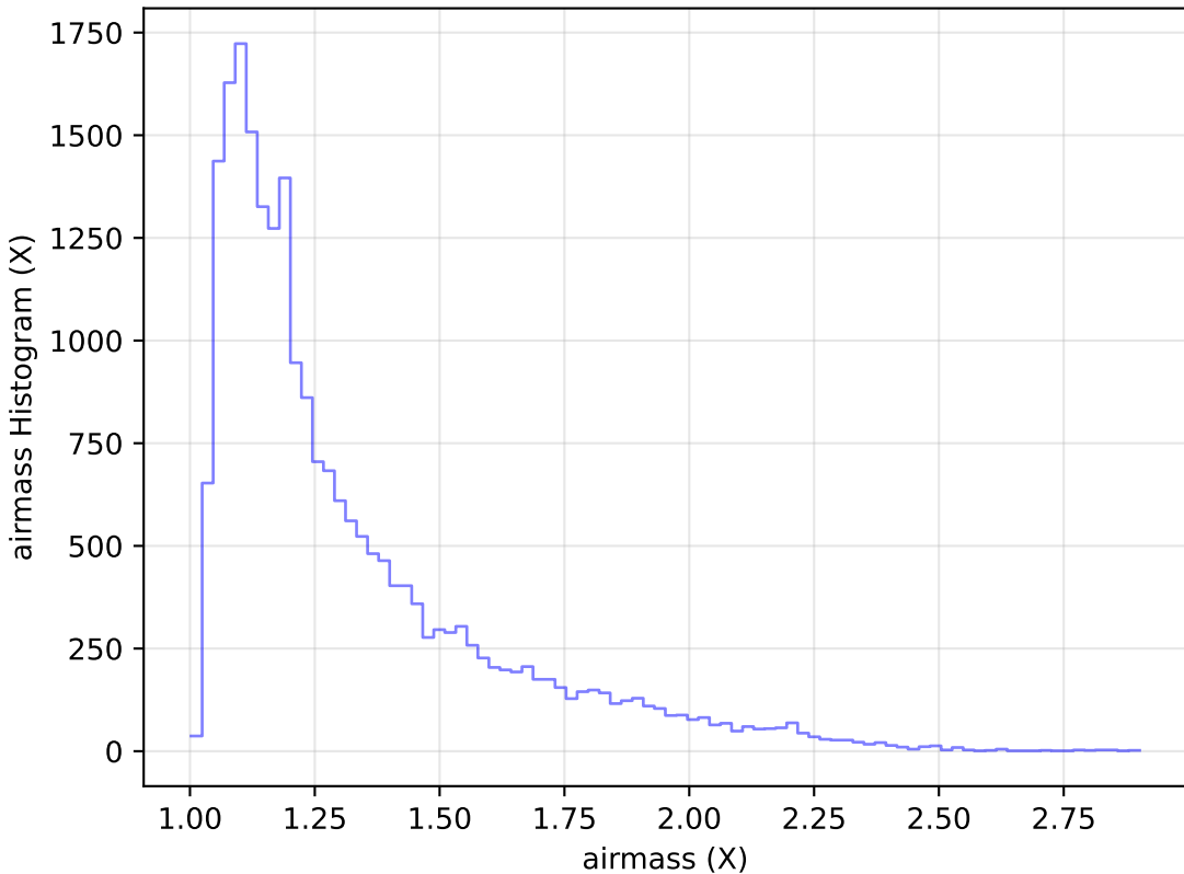
extra_ss_neo2_v3.4_10yrs Yr 1 g band: airmass Histogram
