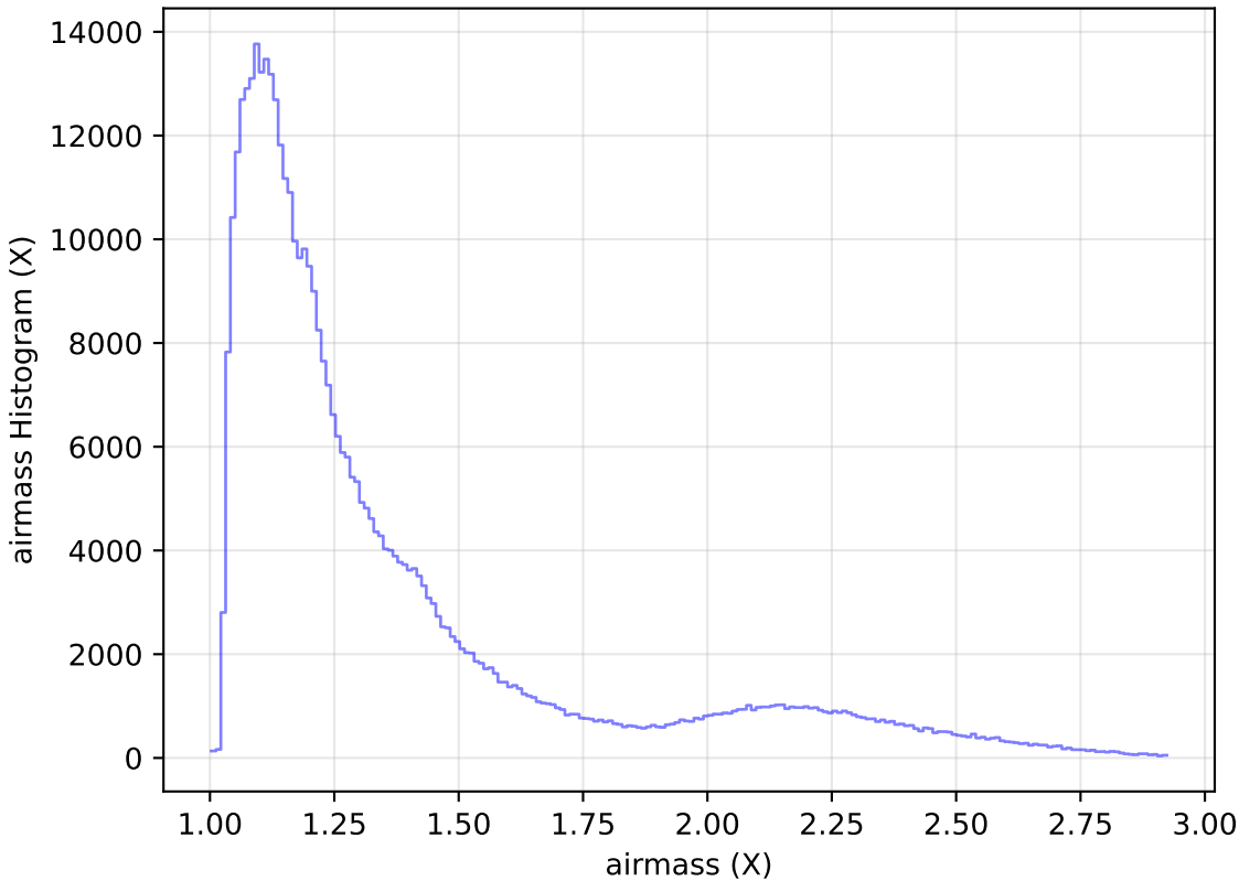
extra_ss_neo2_v3.4_10yrs WFD z band: airmass Histogram
