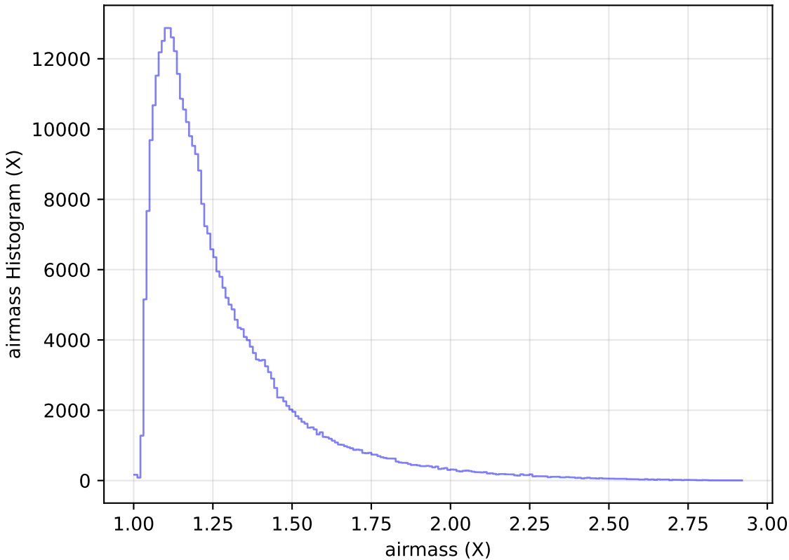
extra_ss_neo2_v3.4_10yrs WFD y band: airmass Histogram
