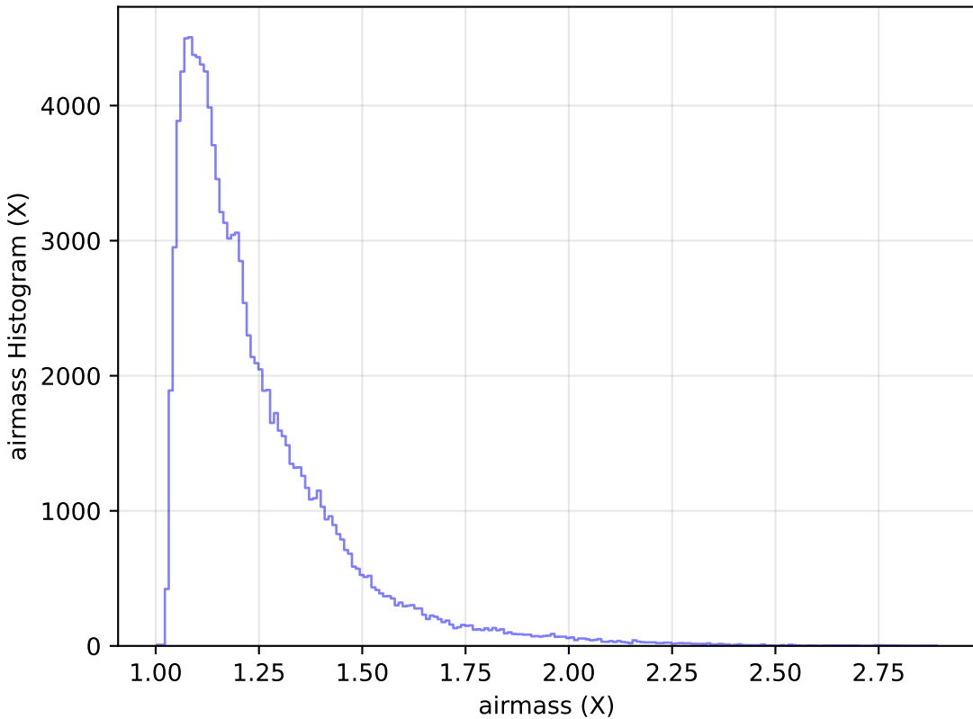
extra_ss_neo2_v3.4_10yrs WFD u band: airmass Histogram
