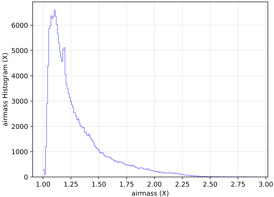
extra_ss_neo2_v3.4_10yrs WFD g band: airmass Histogram
