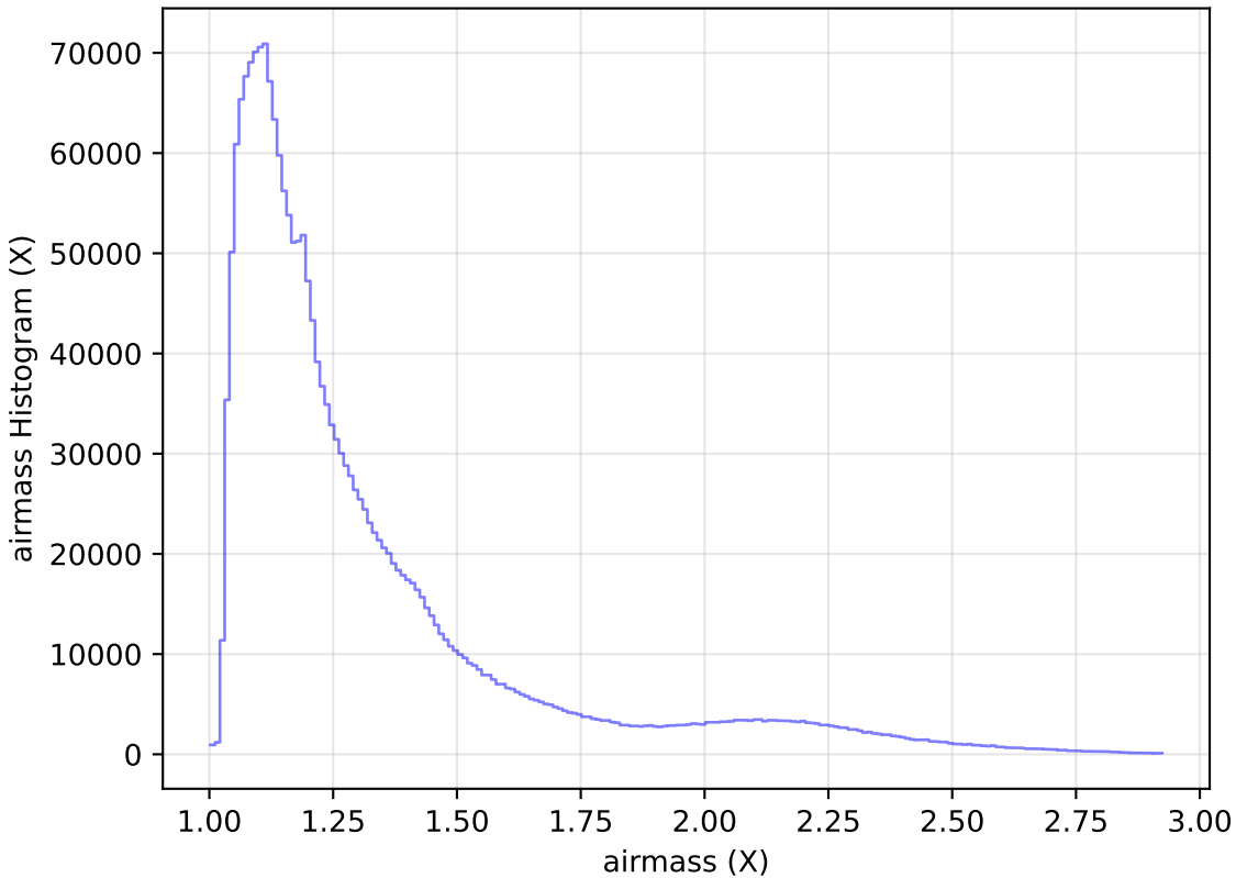
extra_ss_neo2_v3.4_10yrs WFD all bands: airmass Histogram
