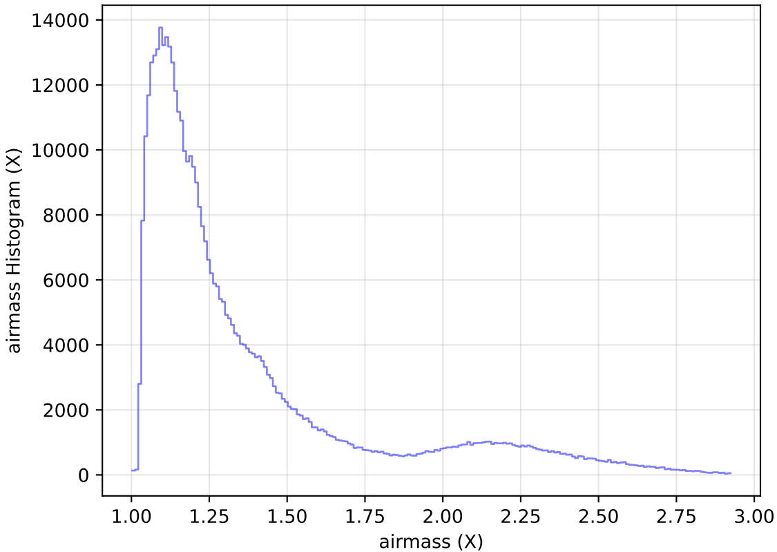
extra_ss_neo2_v3.4_10yrs All sky z band: airmass Histogram
