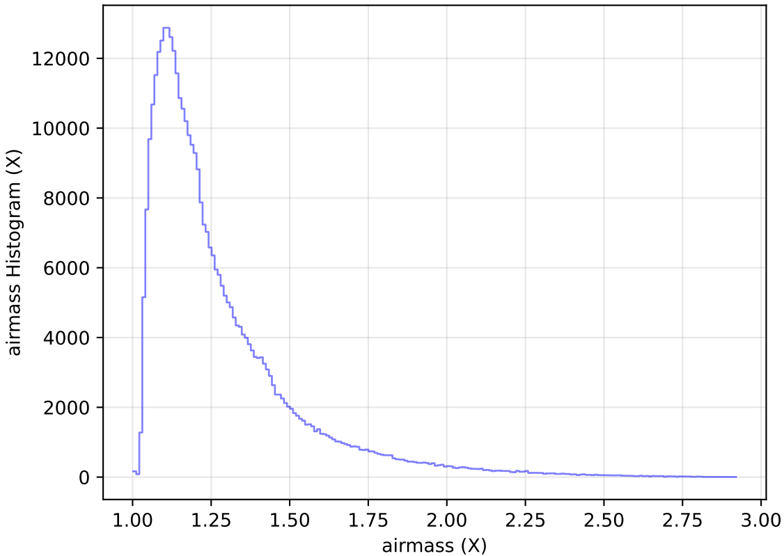
extra_ss_neo2_v3.4_10yrs All sky y band: airmass Histogram
