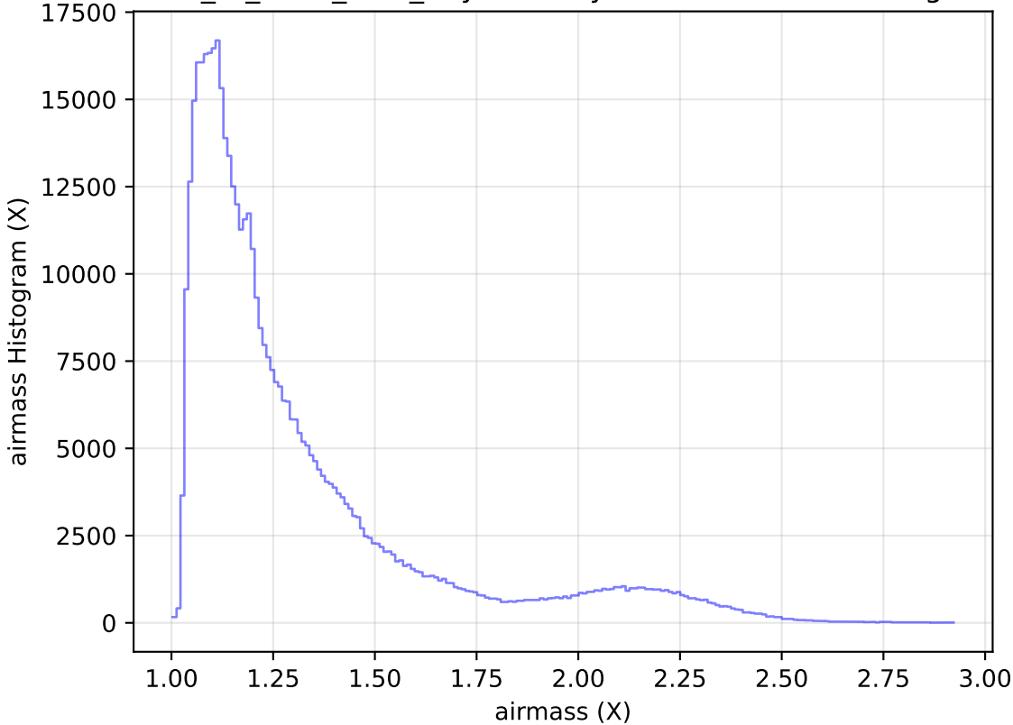
extra_ss_neo2_v3.4_10yrs All sky r band: airmass Histogram
