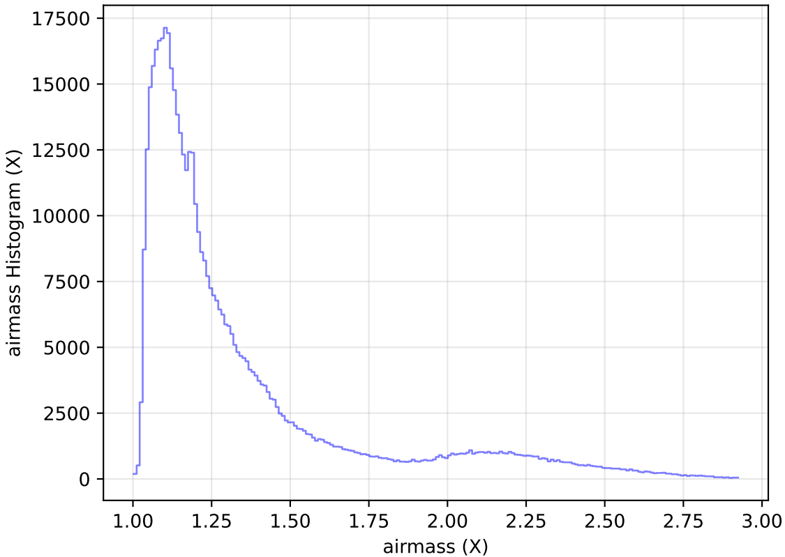
extra_ss_neo2_v3.4_10yrs All sky i band: airmass Histogram
