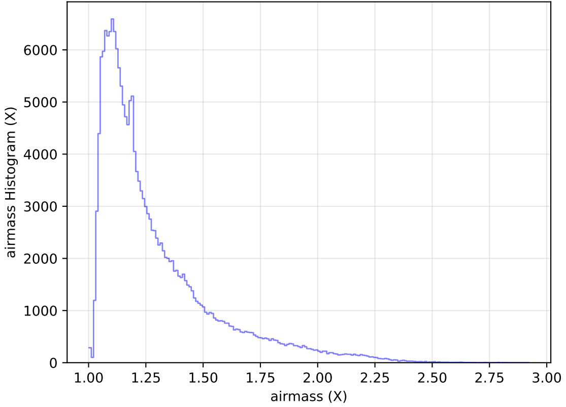
extra_ss_neo2_v3.4_10yrs All sky g band: airmass Histogram
