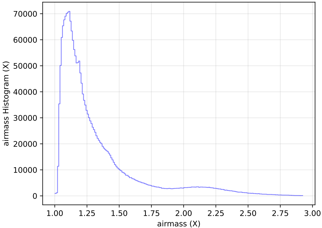
extra_ss_neo2_v3.4_10yrs All sky all bands: airmass Histogram
