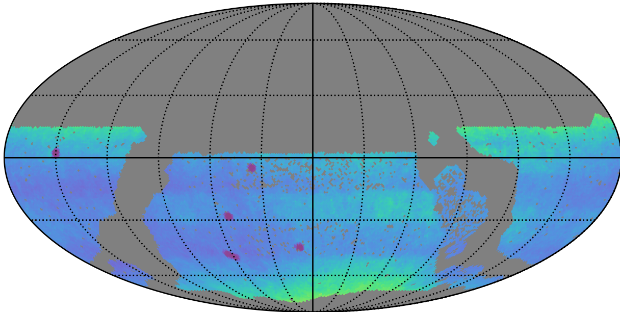
extra_ss_neo2_v3.4_10yrs WFD: Proper Motion Uncert @ 24.0
