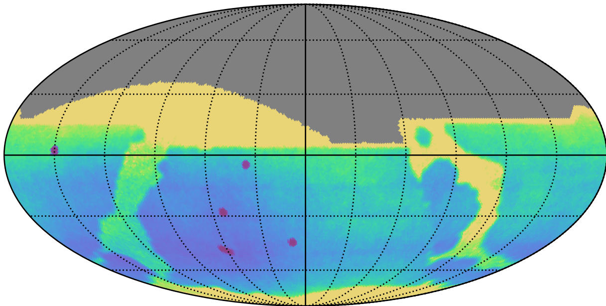
extra_ss_neo2_v3.4_10yrs All sky: Parallax Uncert @ 24.0
