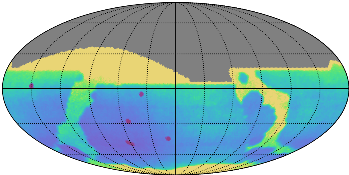
extra_ss_neo2_v3.4_10yrs All sky: Parallax Uncert @ 22.4
