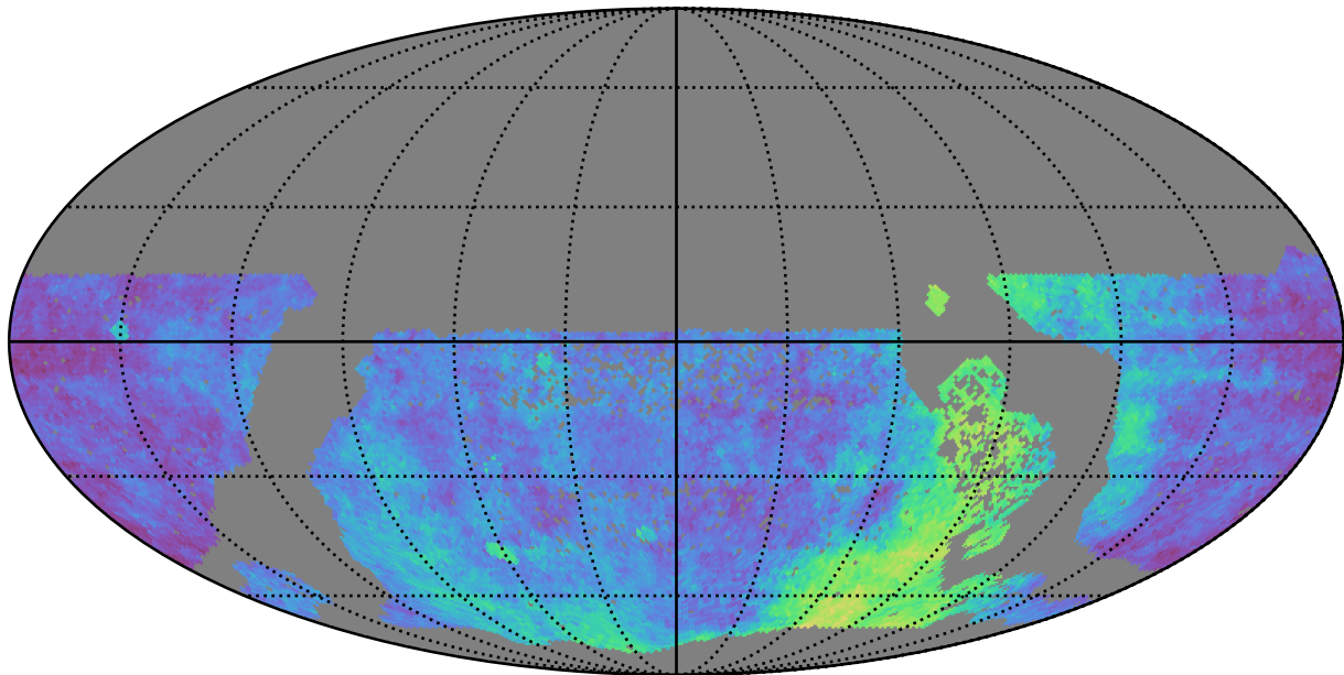
extra_ss_neo2_v3.4_10yrs WFD: Parallax Coverage @ 24.0
