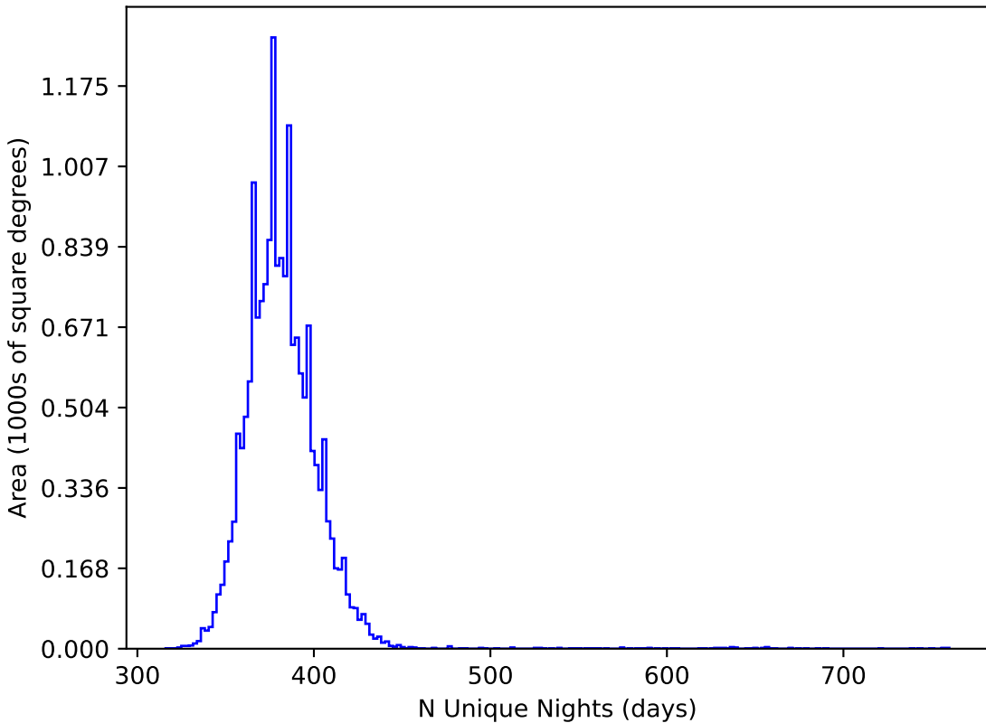
extra_ss_neo2_v3.4_10yrs WFD all bands: N Unique Nights
