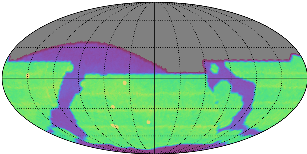
extra_ss_neo2_v3.4_10yrs All sky all bands: N Unique Nights
