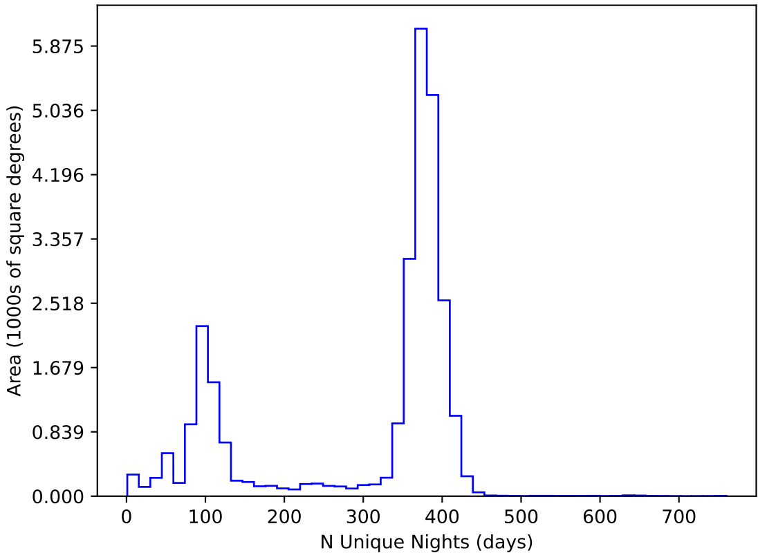
extra_ss_neo2_v3.4_10yrs All sky all bands: N Unique Nights
