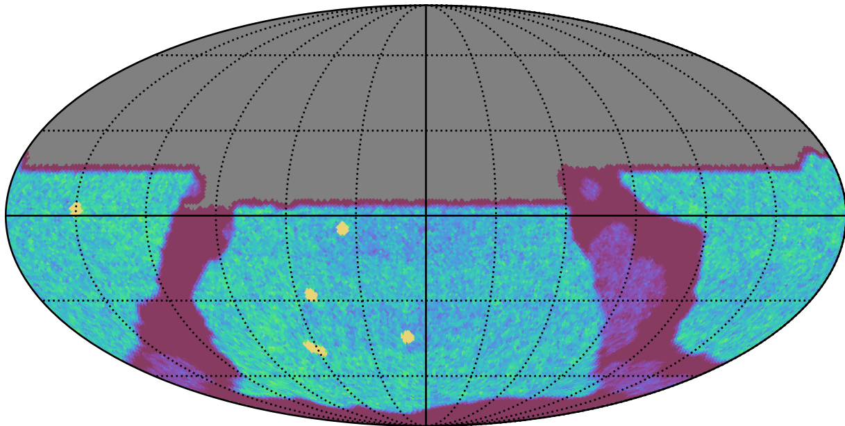
extra_ss_neo2_v3.4_10yrs All sky u band: NVisits
