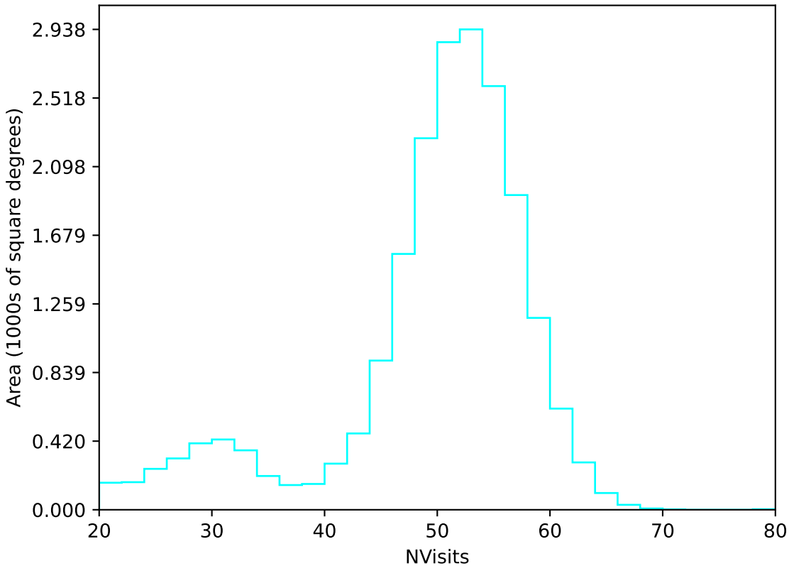
extra_ss_neo2_v3.4_10yrs All sky u band: NVisits
