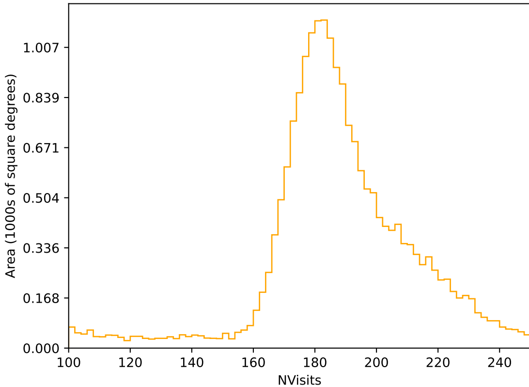
extra_ss_neo2_v3.4_10yrs All sky r band: NVisits
