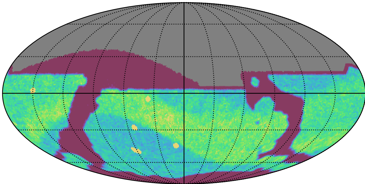
extra_ss_neo2_v3.4_10yrs All sky i band: NVisits
