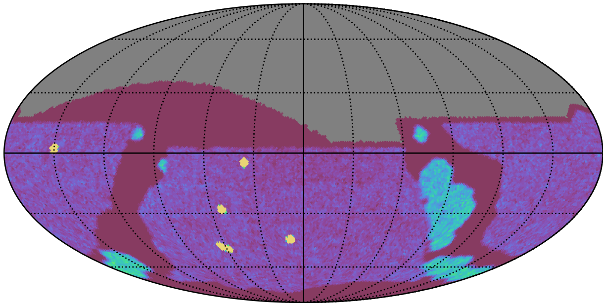
extra_ss_neo2_v3.4_10yrs All sky g band: NVisits
