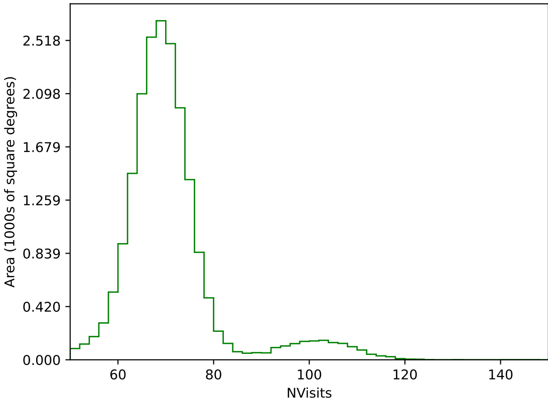
extra_ss_neo2_v3.4_10yrs All sky g band: NVisits
