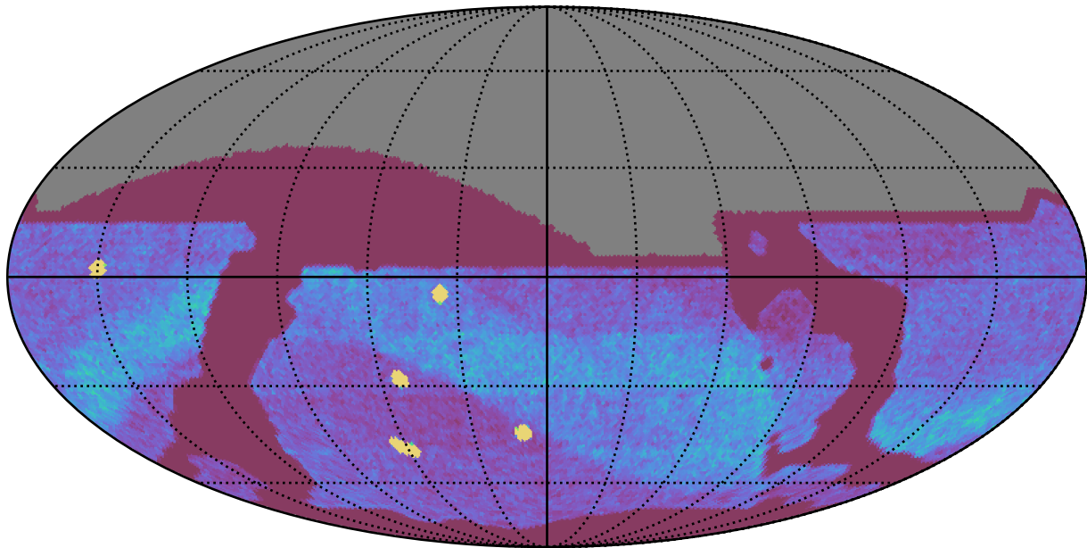
extra_ss_neo2_v3.4_10yrs All sky all bands: NVisits
